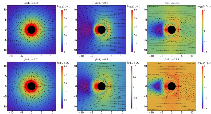
Schwarzschild black hole moving through a cloud of gas (PM and Odrzywolek 2021, 2022)
